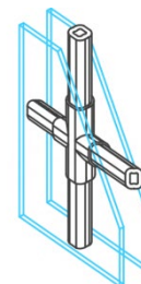
PETIT BOIS INTEGRE 9/5 - GERMANELLA
