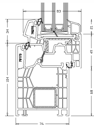
Version semi-affleurant
